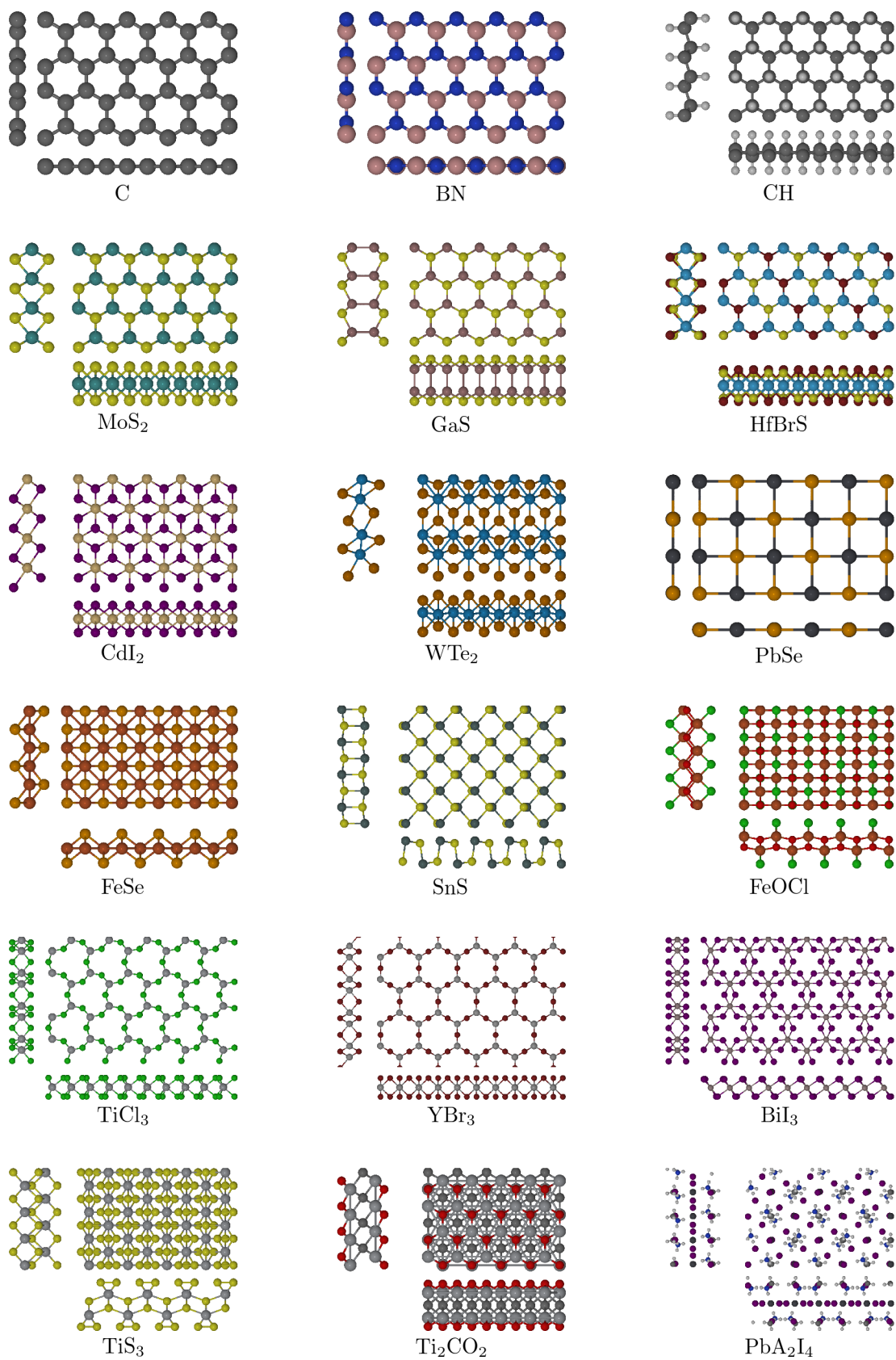
Figure 4: Examples of crystal structure prototypes currently included in the C2DB.
