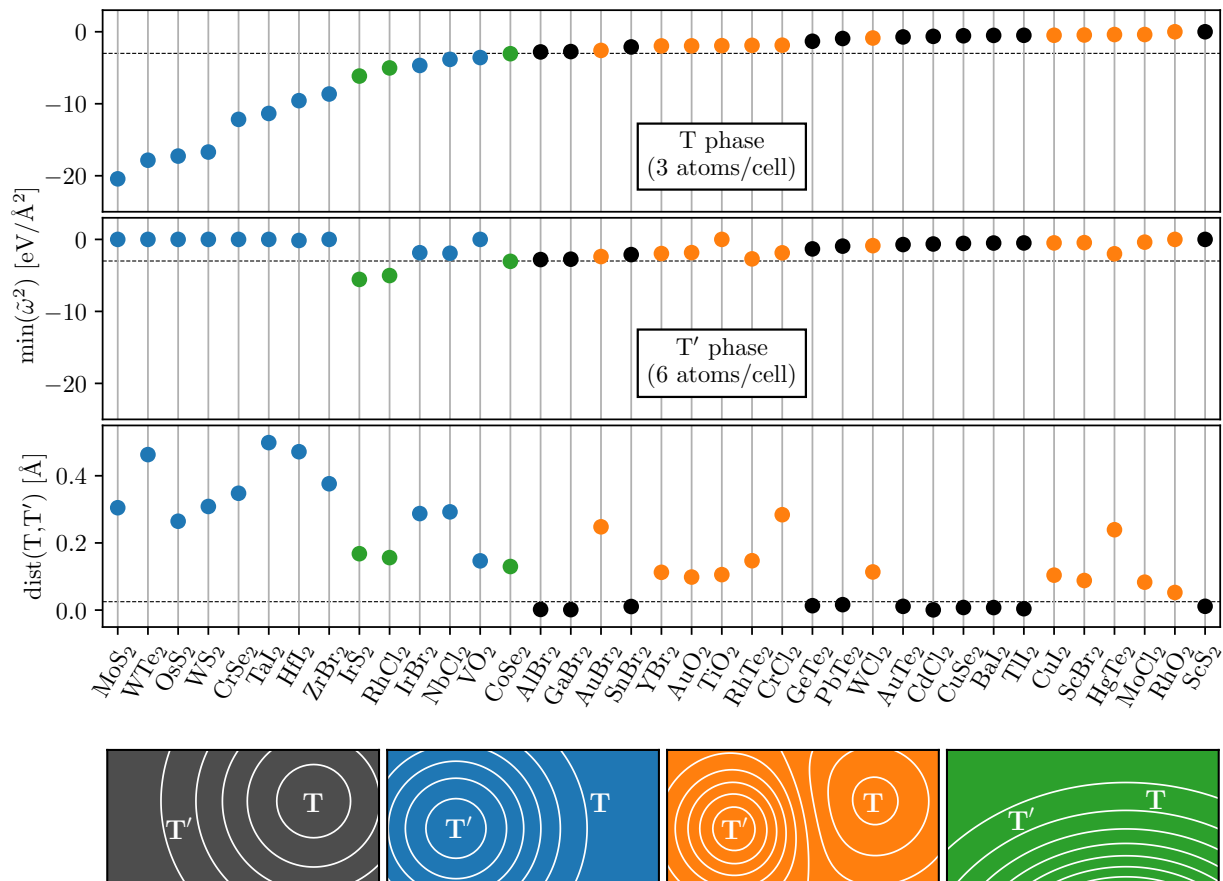
Figure 6: Dynamical stability of a set of transition metal dichalcogenides and -oxides in the T and T' phases ( \text{CdI}_2 and \text{WTe}_2 prototypes), respectively. The first and second panels show the minimum eigenvalue of the \Gamma -point dynamical matrix of the 2 \times 2 unit cell (containing 12 and 24 atoms for the T and T' phase, respectively). The lower panel shows the root mean square distance (RMSD) between the relaxed structures. The color indicates whether the material is dynamically stable in the T phase (black), the T' phase (blue), both phases (orange) or neither of the phases (green).
