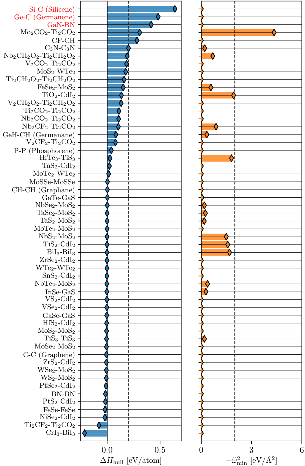
Figure 7: The calculated energy above the convex hull and minimum eigenvalue of the dynamical matrix (evaluated at the \Gamma -point for the 2 \times 2 cell) for the 55 materials in the C2DB that have been synthesised or exfoliated in monolayer form, see Refs. 6,9,10,12,50–57,57–95. The three materials highlighted in red have only been synthesised on metallic substrates. The black dashed lines indicate the thresholds used to categorise the thermodynamic and dynamical stability of materials in the C2DB.
