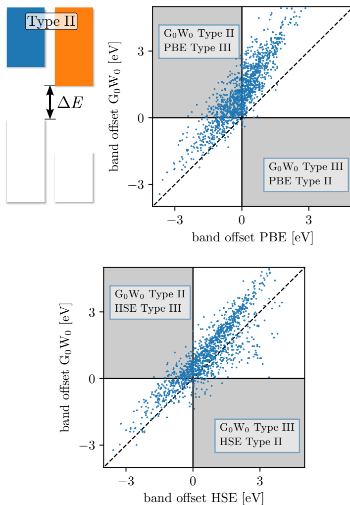
Figure 21: Band alignment at heterobilayers, assuming that the bands line up with a common vacuum level. The left panel shows the definition of the band offset \Delta E . The middle and right panels show randomly selected bilayer combinations with Type II ( \Delta E > 0 ) or Type III ( \Delta E < 0 ) band alignment. The black line indicates the bisector, the grey areas indicate qualitatively wrong DFT band alignments compared to G_0W_0 .
