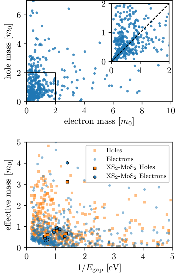
Figure 22: (left) Effective electron mass versus hole mass. On average holes are slightly heavier than electrons. (right) Effective carrier mass versus the inverse band gap. The linear correlation between the two quantities, expected from \mathbf{k} \cdot \mathbf{p} perturbation theory, is seen not to hold in general. Materials with the formula XS 2 in the MoS 2 crystal structure are highlighted.
