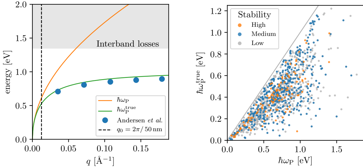
Figure 25: (left) Plasmon dispersion relations for the unscreened (i.e. intraband) and true plasmons, \hbar\omega_{\text{P}} and \hbar\omega_{\text{P}}^{\text{true}} , respectively, for NbS 2 in the H phase (the MoS 2 crystal structure prototype). This is compared to the full first principles calculations of the plasmons in NbS 2 by Andersen et al. (data points). 165 (right) The in-plane averaged true plasmon frequency versus the unscreened plasmon frequency for all metals in C2DB at a plasmon wavelength of \lambda_{\text{P}} = 50 nm corresponding to q_0 in the left panel. The data points are colored by the overall stability level as defined in Section 2.4.1, and the straight line corresponds to \hbar\omega_{\text{P}} = \hbar\omega_{\text{P}}^{\text{true}} .
