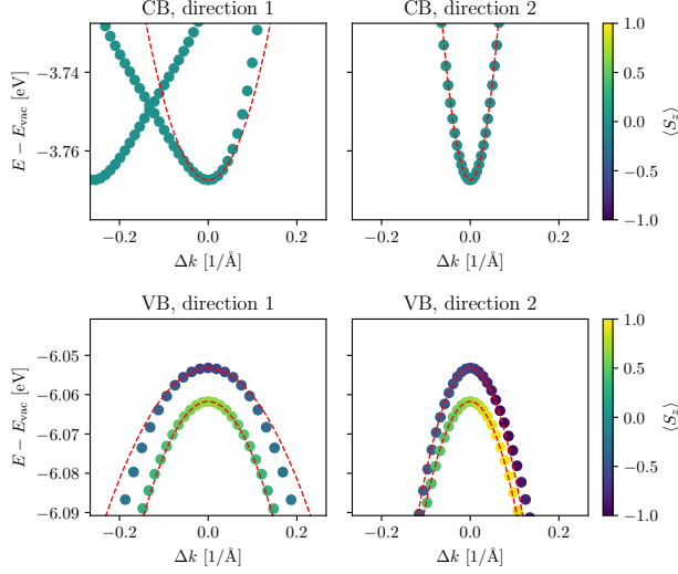
Figure 14: Zoom of the band structure of SnS in the GeSe crystal structure around the conduction and valence band extrema (upper and lower panels). Second order fits used to determine the effective masses are shown by red dashed lines. The peculiar band splitting in the conduction band minimum (upper left panel) is caused by a Rashba effect arising from the combination of spin-orbit coupling and the finite perpendicular electric field created by the asymmetric SnS structure.
