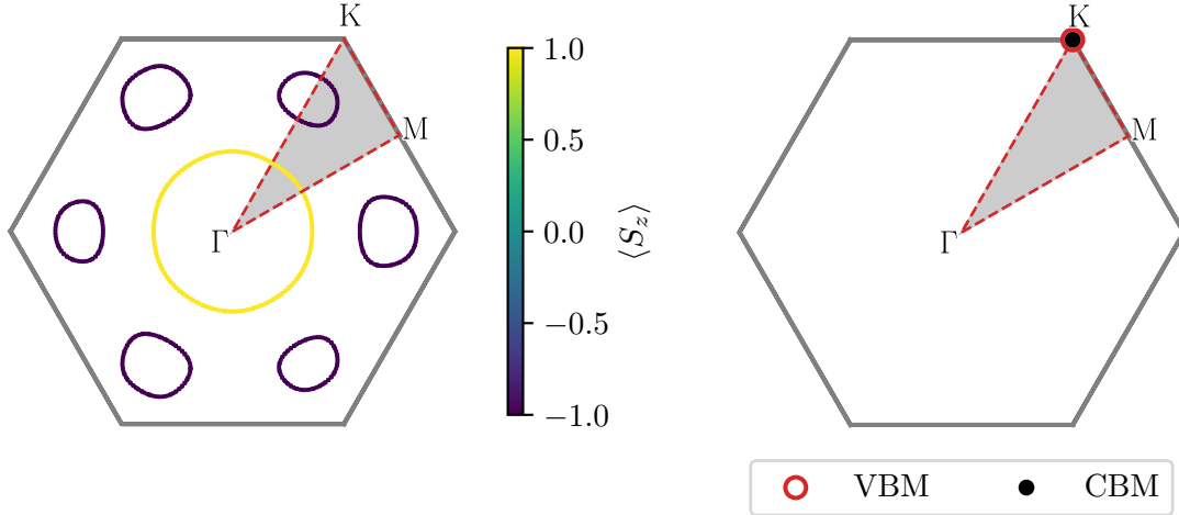
Figure 13: Left: Brillouin zone and Fermi surface calculated with PBE and spin-orbit coupling for \text{VO}_2 in the \text{MoS}_2 crystal structure. The Fermi surface is colored by the spin projection along the z -axis. Right: Brillouin zone, valence band maximum (VBM) and conduction band minimum (CBM) for \text{WS}_2 in the \text{MoS}_2 crystal structure. The grey areas in both plots mark the irreducible Brillouin zone.
